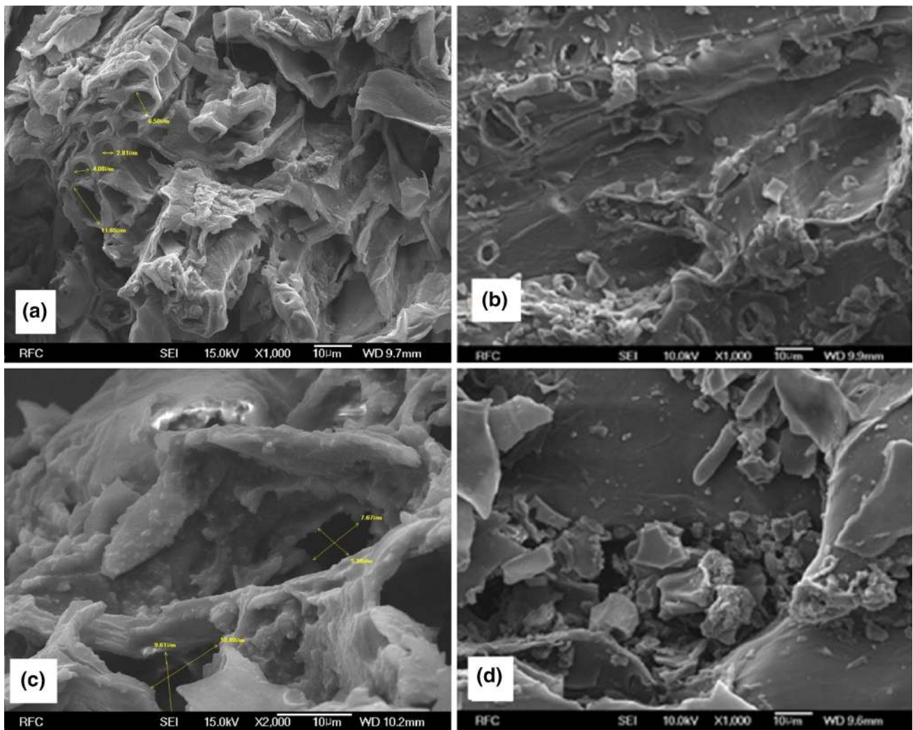
Fig. 3 The SEM micrographs of raw PC biochar samples before and after adsorption of arsenic(III) (a, b), and Zn-loaded PC biochar samples before and after adsorption of arsenic (III) (c, d), respectively
