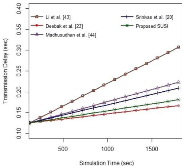
Fig. 3 Transmission Delay (sec)
