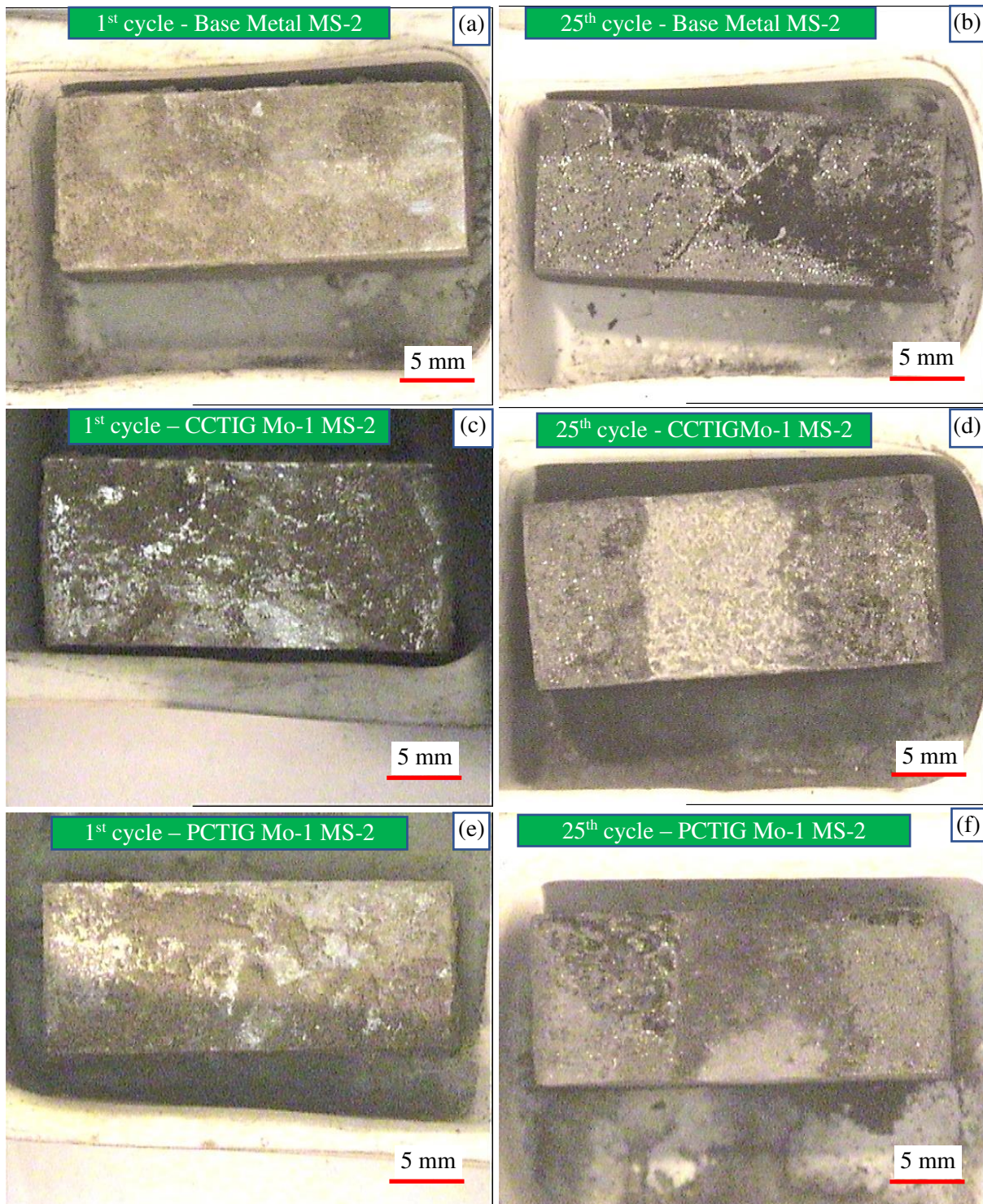
Figure 2. Macrostructure of the hot corrosion samples in MS-2 ( 70\text{Na}_2\text{SO}_4 + 25\text{V}_2\text{O}_5 ); (a) Base Metal – Before 1 st cycle, (b) Base Metal – After 25 th cycle, (c) CCTIG Mo-1 - Before 1 st cycle, (d) CCTIG Mo-1 - After 25 th cycle, (e) PCTIG Mo-1 - Before 1 st cycle (f) PCTIG Mo-1 - After 25 th cycle.
