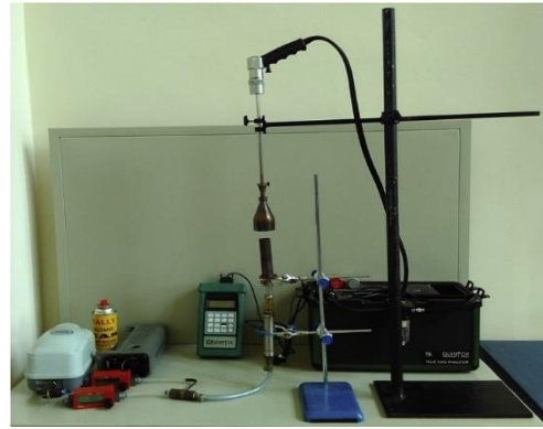
Figure 3. Experimental burner setup.
