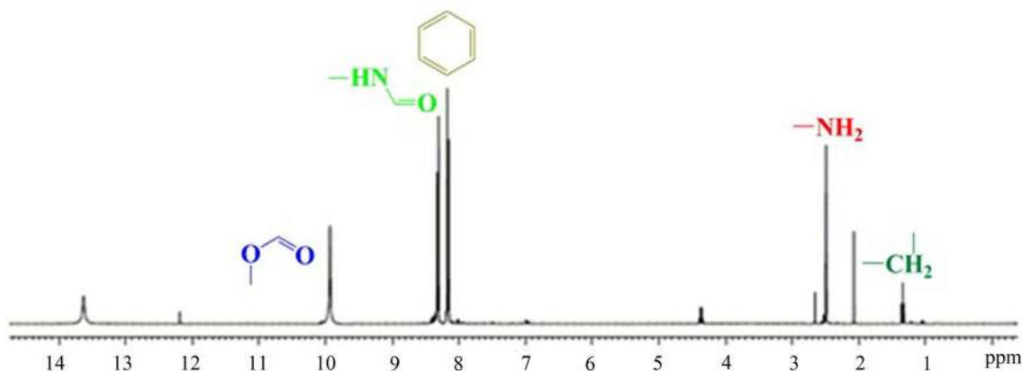
Fig. 4 Proton magnetic resonance spectrum of Folic acid-PEG-DSPE conjugate
