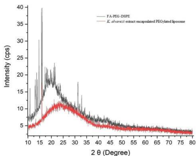
Fig. 5 XRD pattern of folic acid-PEG-DSPE conjugate and K. alvarezii extract-encapsulated FA-conjugated PEGylated liposome
