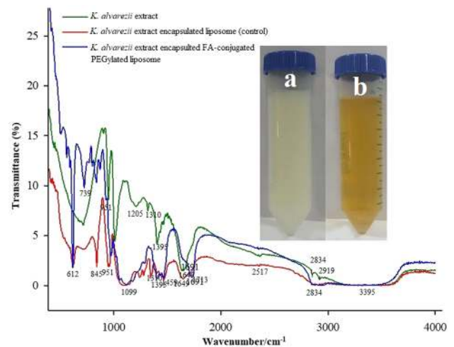
Fig. 2 FT-IR spectra of K. alvarezii extract, K. alvarezii extract-encapsulated PEGylate liposome, K. alvarezii extract-encapsulated FA-conjugated PEGylate liposome
