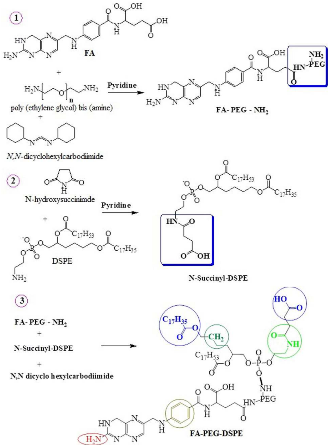
Fig. 1 Synthetic scheme of folic acid-PEG-DSPE conjugate
