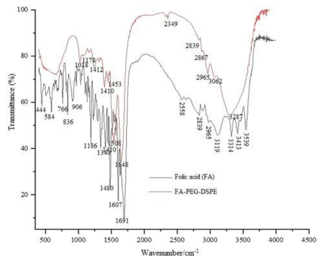
Fig. 3 FT-IR spectra of FA and folic acid-PEG-DSPE conjugate
