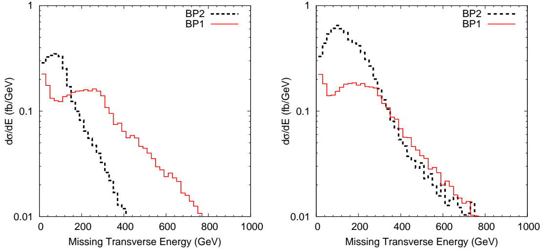
FIG. 3: (a) \cancel{E}_T for doubly-charged Right-handed Higgsino and Higgs boson, (b) \cancel{E}_T for doubly-charged Right-handed and Left-handed Higgsinos and Right-handed Higgs boson.
