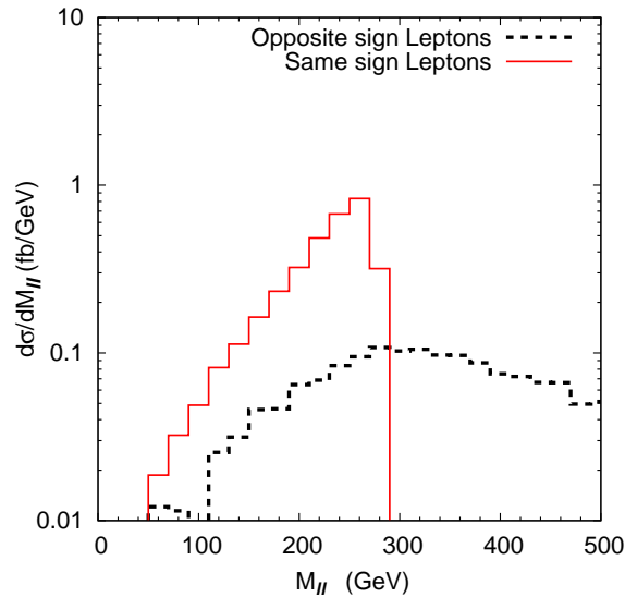
FIG. 6: Invariant mass distribution in M_{ll} for a doubly-charged right-handed Higgsino which decays through an off-shell doubly-charged Higgs boson.
