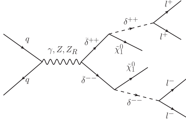
FIG. 1: Direct production of \tilde{\delta}_R^{\pm\pm} pair at the LHC. Subsequent decays of \tilde{\delta}_R^{\pm\pm} give rise to two leptons plus missing energy signal, if M_{\tilde{\delta}_R^{\pm\pm}} < M_{\tilde{\chi}_1^0} .
