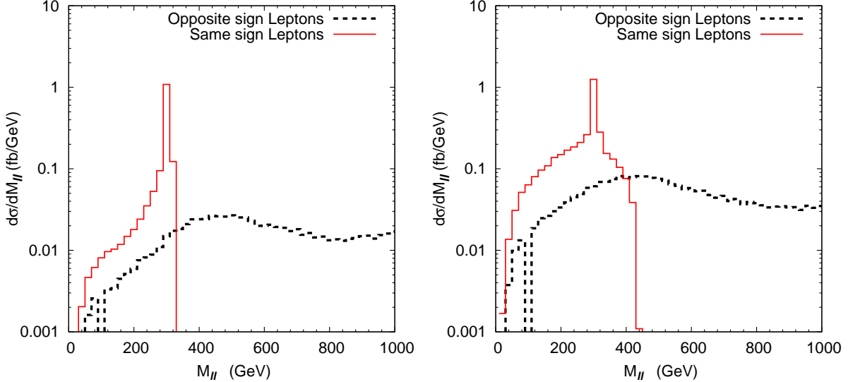
FIG. 5: Illustrating the (a) invariant mass distribution for events coming from the doubly-charged right-handed Higgsino and Higgs boson pair production and, (b) invariant mass distribution for events when the contributions from the pair production of the left-handed Higgsinos is also included for BP1 .
