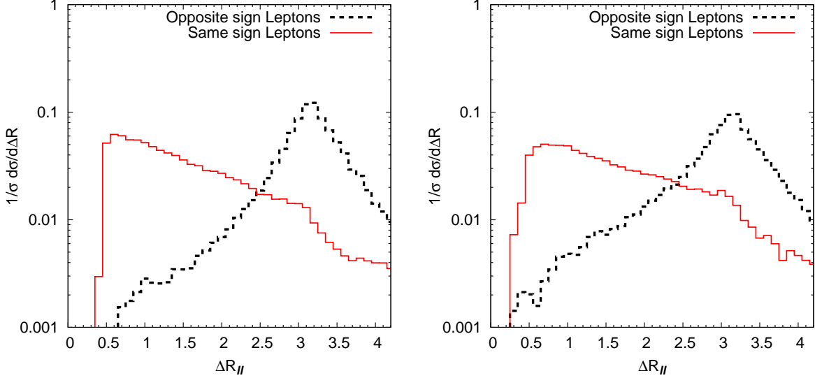
FIG. 4: (a) Illustrating the \Delta R_{ll} distribution for events coming from the doubly-charged right-handed Higgsino and Higgs boson pair production and, (b) \Delta R_{ll} distribution for events when the contributions from the pair production of the left-handed Higgsinos is also included for BP1 .
