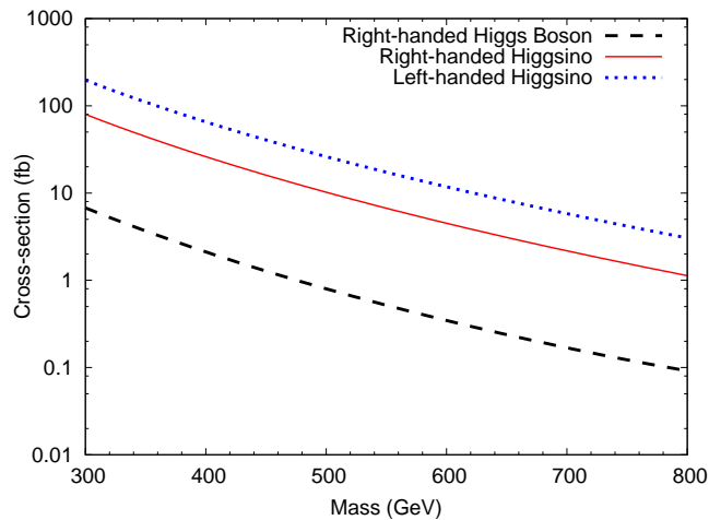
FIG. 2: Production cross sections for \tilde{\delta}_{L,R}^{\pm\pm} pair and \delta_R^{\pm\pm} at the LHC at 14 TeV
