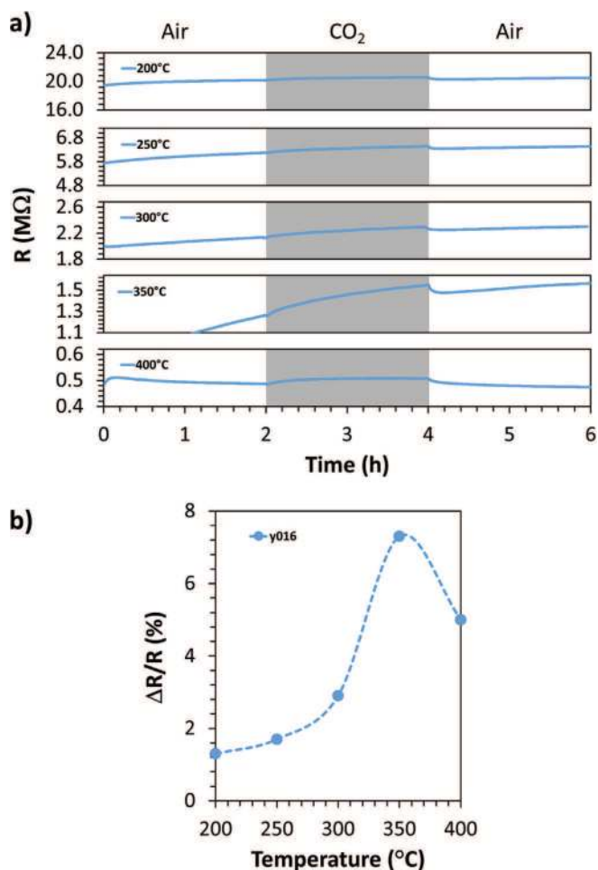
Fig. 6. For the y016 sample: a) resistance in the presence of air ( R_{air} ) and CO 2 ( R_{CO_2} ) in the 200–400 °C temperature range and b) \Delta R/R_{air} with at various operating temperature.
