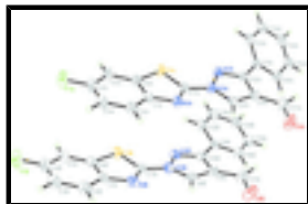
Fig. 1. The molecular structure of the title compound, showing two independent molecules with atom labels and 30% probability displacement ellipsoids.
