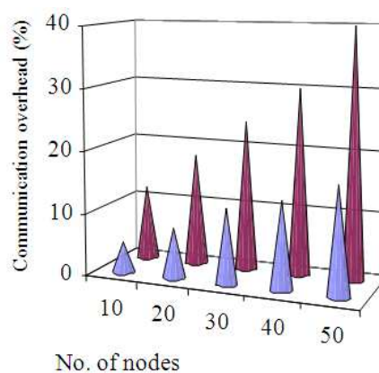
Fig. 7. Clustered nodes Vs. Communication overhead
