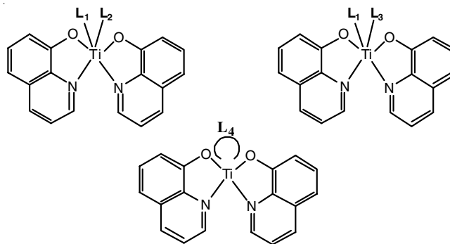
Fig. 2. Proposed structures of the titanium(IV) derivatives
