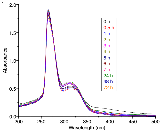
Fig. 1. UV-visible absorption overtime for 2-acetyl-5-furanoximate-2-methoxyethanolato-bis(8-quinolinato)titanium(IV)] (3d) upon addition of water
