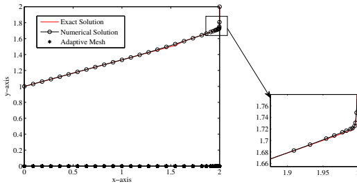
Figure 1. Numerical solution for Example 1 with \varepsilon = 2^{-8} , N = 23 (initially)
