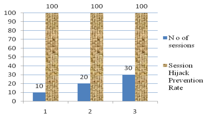
Fig. 9. Session Hijack prevention rate for 212 chars encrypted session ID
