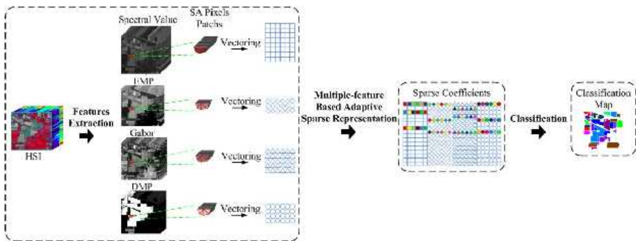
Figure. 1. MFASR Architecture
