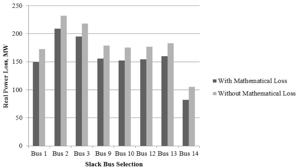
Figure 3. Transmission loss with and without mathematical loss for IEEE 75 bus system
