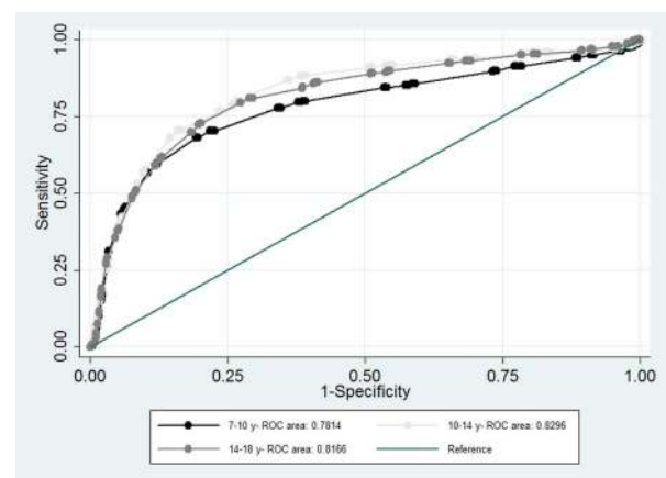
Figure 2 Receiver operating characteristic curve of neck circumference for predicting overweight in Iranian children and adolescents by age categories. ROC, receiver operating characteristic.
