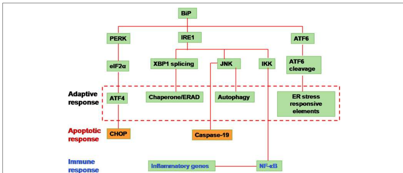
FIGURE 1 | Unfolded protein response signaling. The signaling is initiated by the activation of the proximal sensors of the unfolded protein response (UPR) namely, (1) protein kinase R (PKR)-like ER kinase (PERK), (2) activating transcription factor (ATF) 6 and (3) inositol-requiring enzyme 1 (IRE1). A protein called immunoglobulin heavy chain binding protein (BiP) functions as the master regulator. BiP under normal conditions remains attached to all the three sensors in the luminal domain of the endoplasmic reticulum (ER). Upon encountering any stress like accumulation of misfolded/unfolded proteins or a massive inflow of any exogenous proteins into the ER, the stress sensors, PERK, IRE1, and ATF6, are activated by the release of BiP from the sensors leading to any of the three distinct pathways. (1) When PERK is activated, it dimerises and autophosphorylates leading to phosphorylation of the eukaryotic translation initiation factor (eIF) 2 \alpha . Activated eIF2 \alpha represses global protein translation of the cell. However the downstream protein called ATF 4 can escape translational repression since it has upstream open reading frames leading to its activation. The activated ATF4 translocates into the nucleus activating a set of target genes to restore cellular homeostasis (adaptive response). However in situations when the cellular homeostasis cannot be restored, C/EBP
