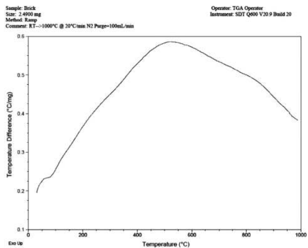
Figure 8: DTA curve of the brick sample
