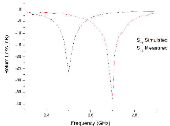
Figure 4: Simulated and measured return loss (dB)
