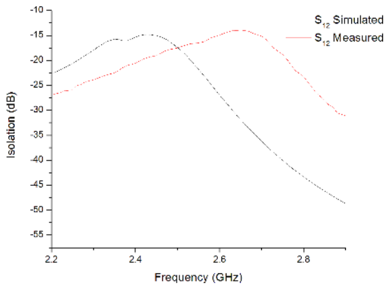
Figure 5: Simulated and measured Isolation (dB)
