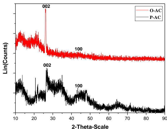
Figure 5. XRD peaks for P-AC and O-AC.
