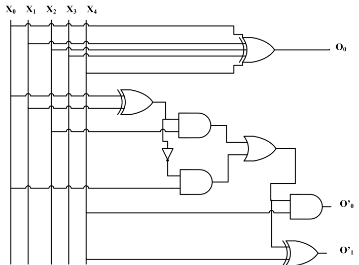
FIGURE 2: Logic diagram of design 2 approximate 5-3 compressor
