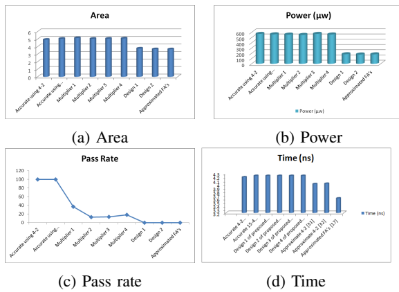
FIGURE 8: Graphical representation of 16 \times 16 bit multiplier results
