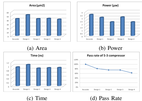
FIGURE 6: Graphical representation of 5-3 compressor results
