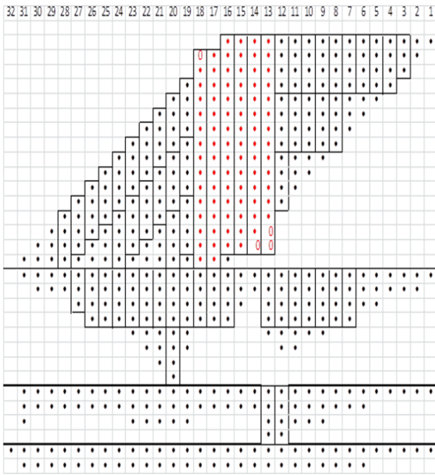
FIGURE 5: Design of 16 \times 16 Multiplier using 15-4 compressor
