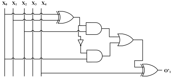
FIGURE 3: Logic diagram of output O'_1
