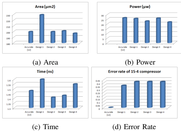
FIGURE 7: Graphical representation of 15-4 compressor results
