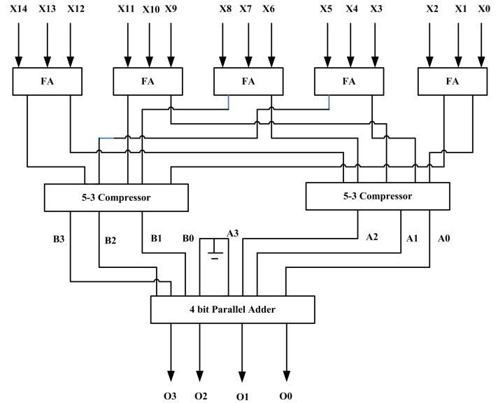
FIGURE 4: Design of accurate 15-4 compressor [12]
