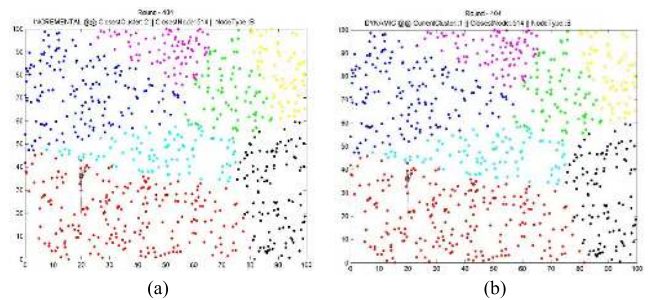
FIGURE 9. Incremental cluster formation observation. (a) Second incremental cluster. (b) Dynamic cluster unchanged.
