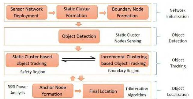
FIGURE 4. Overview of the proposed research.
