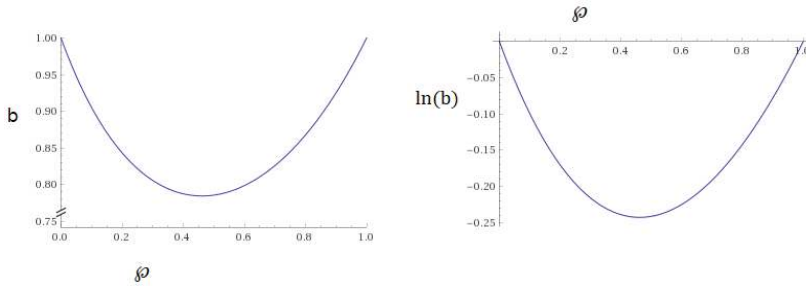
Figure 1. The relation between b = \Gamma^2(\varphi + 1) and \varphi in the left, while the right graph is the relation between \ln(b) = F with respect to \varphi . The minimum value of b is at \varphi = 0.4616 .
