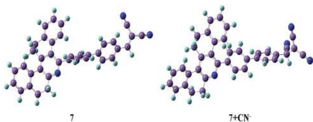
Fig. 13 Optimized structures of 7 and 7 + CN - .
