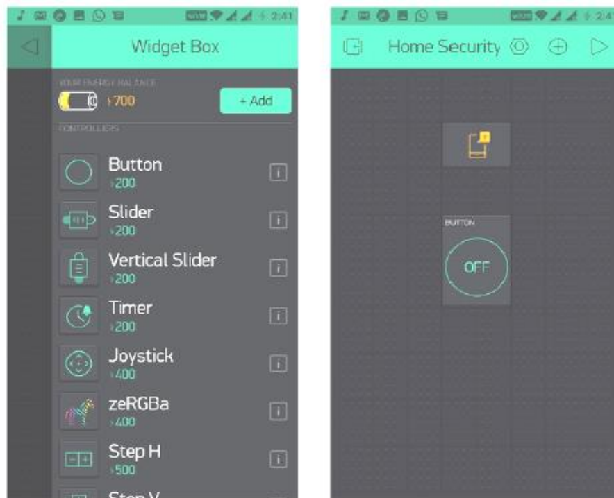
Figure 11. Adding widgets.
