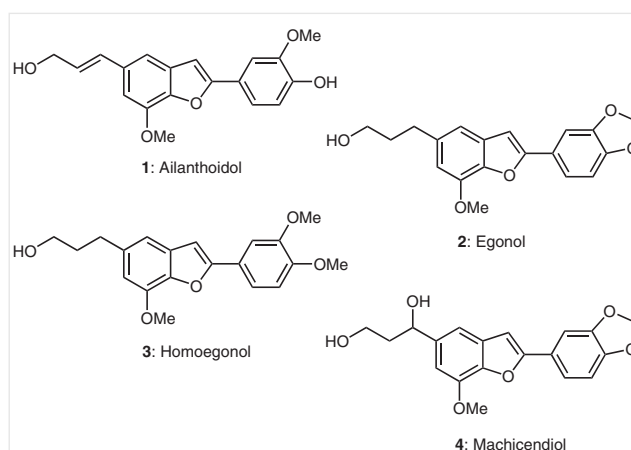
Figure 1 The structures of benzofuran-cored naturally occurring compounds
