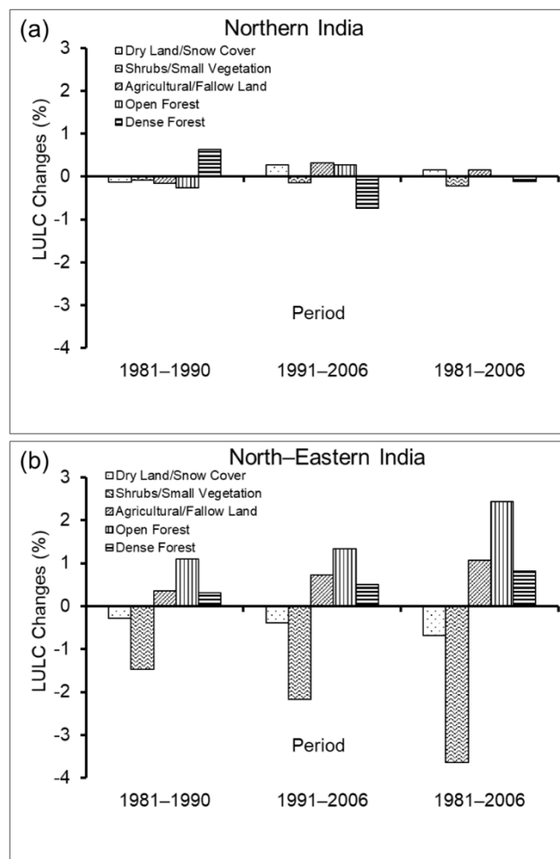
Figure 6. LULC changes over (a) NI and (b) NEI.
