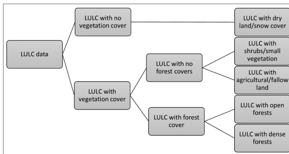
Figure 2. Hierarchy approach used for classification.
