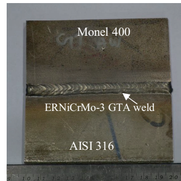
Fig. 1 Macro-photograph of the GTA weldments of Monel 400 and AISI 316
