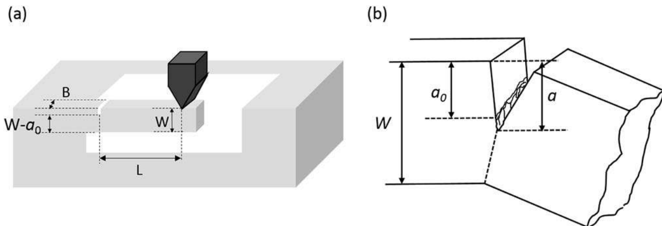
Fig. 1. (a) Schematic of the geometry of the micro-cantilevers prepared by FIB milling. (b) Definition of the crack length.
