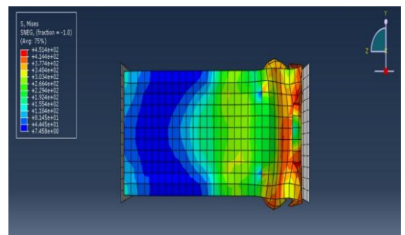
Figure 17. Model 2 steel after crush
