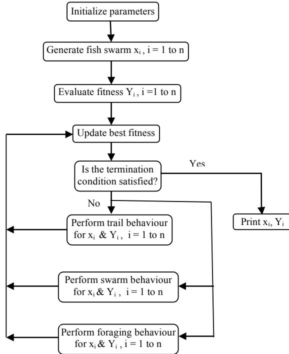
Figure 1. Flow chart of Artificial Fish Swarm algorithm
