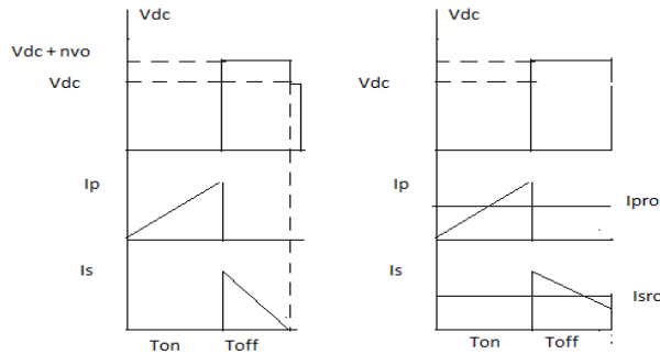
Figure 4. (a) DCM characteristic, (b) CCM characteristic
