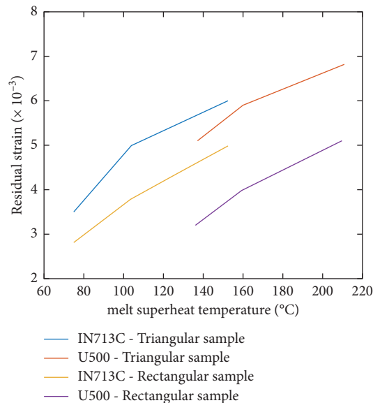
FIGURE 21: Relationship between residual strain and melt superheat temperature.
