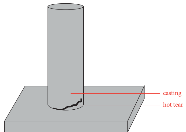
FIGURE 67: Hot crack formed in a cast component.
