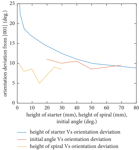
FIGURE 4: Change in orientation deviation w.r.t. changes in height of starter, height of spiral, and initial angle.
