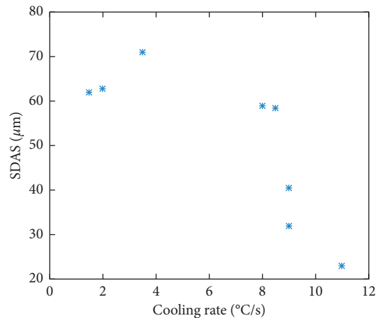
FIGURE 25: Correlation between SDAS and cooling rate.
