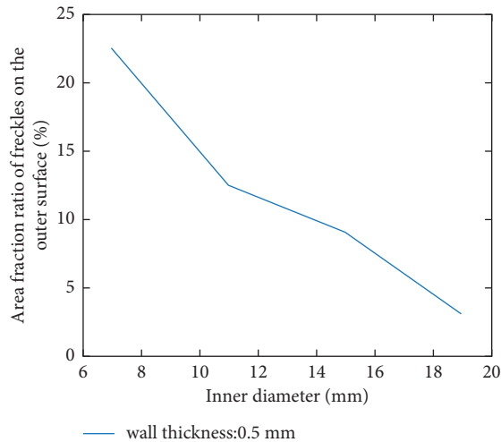
FIGURE 57: A relation between area fraction of freckles on the outer surface and the inner diameter.
