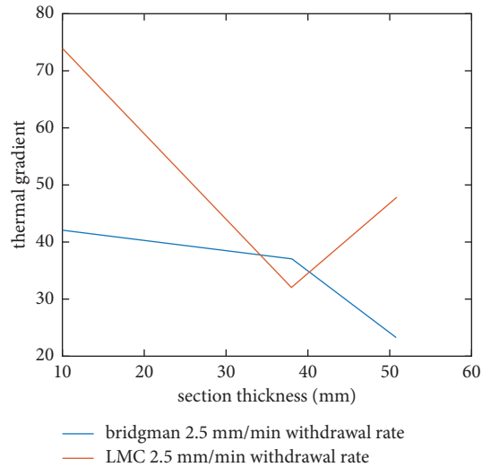
FIGURE 15: Relationship between section thickness and thermal gradient in samples made using different processes.
