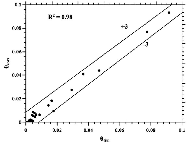
Figure 11. Parity plot showing the agreement between non-dimensional simulated temperature ( \theta_{sim} ) and non-dimensional correlated temperature ( \theta_{corr} ).
