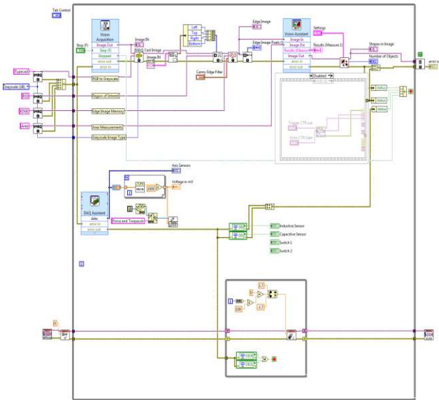
Figure 4. Circuit diagram for sensors integrated platform of Main DAQ VI.vi setup using LabVIEW.
