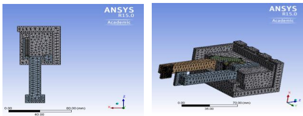
Figure 5. Mesh analysis of robotic hand.
