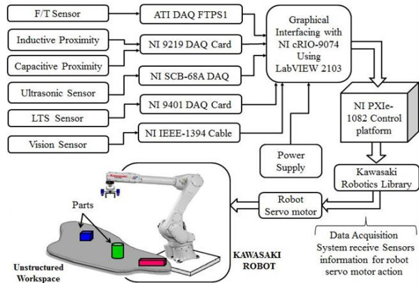
Figure 1. Scheme of sensor integration with DAQ system.
