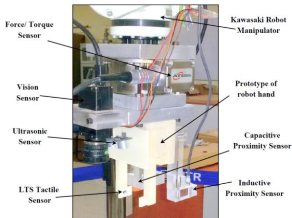
Figure 6. Sensors integrated robotic hand.
