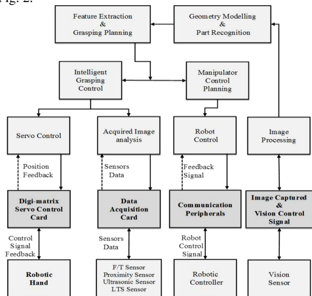
Figure 2. Control system architecture.
