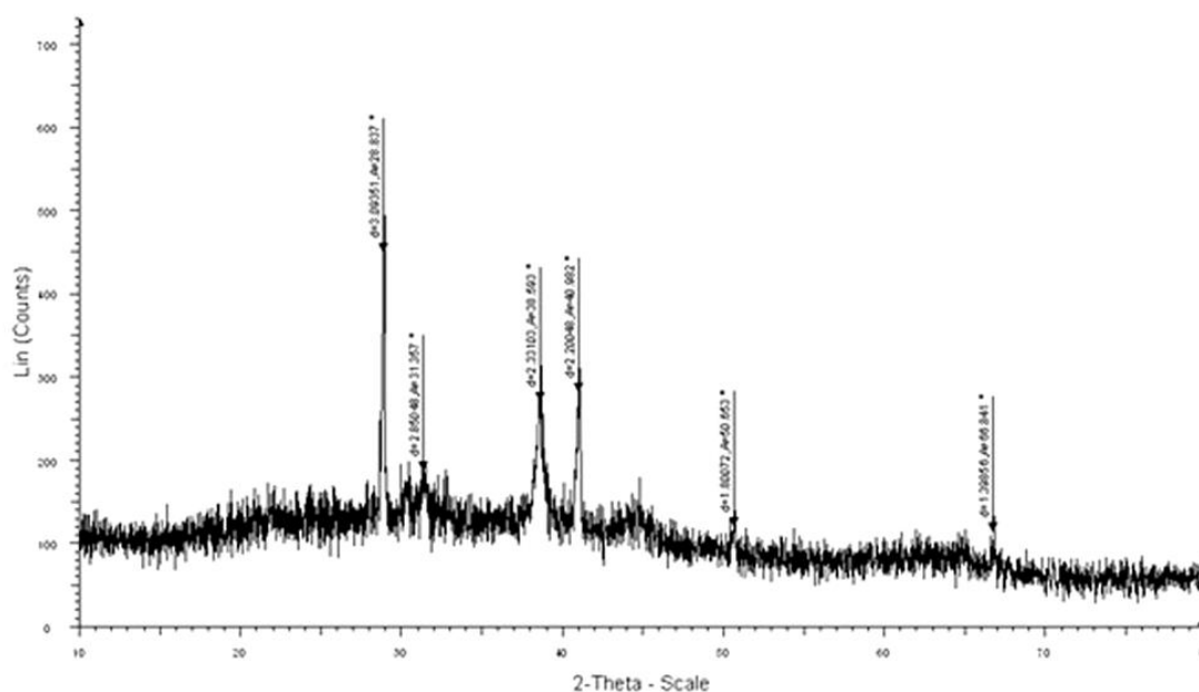
Fig. 5: XRD pattern of AgNPs exhibiting the facets of crystalline silver.
