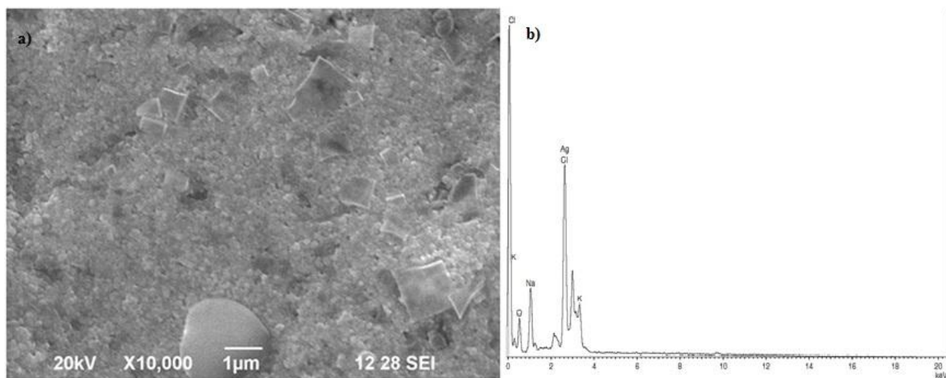
Fig. 3: (a) SEM image of AgNPs and (b) EDX spectrum of AgNPs.
