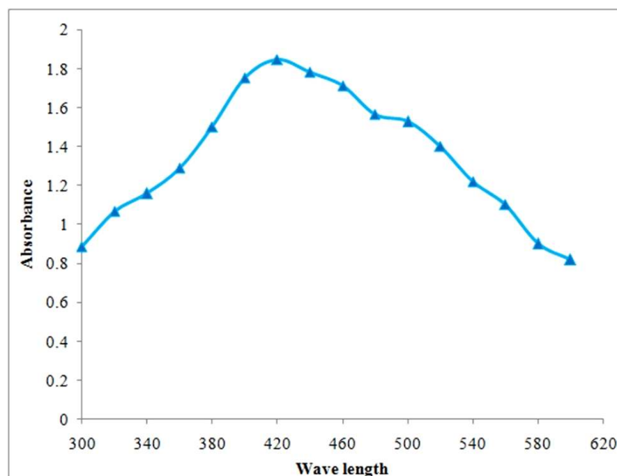
Fig. 1: UV-vis spectra of Cymodocea rotundata extract containing AgNPs.
