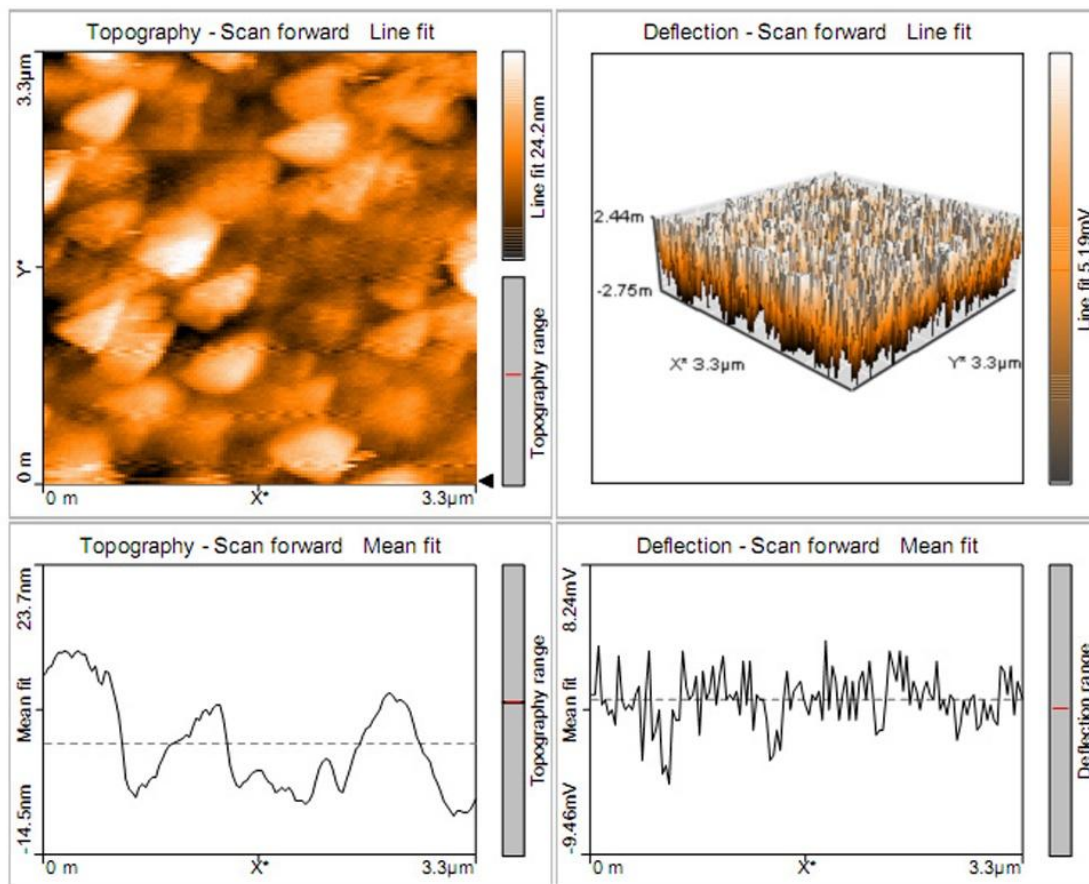
Fig. 2: AFM image of AgNPs.
