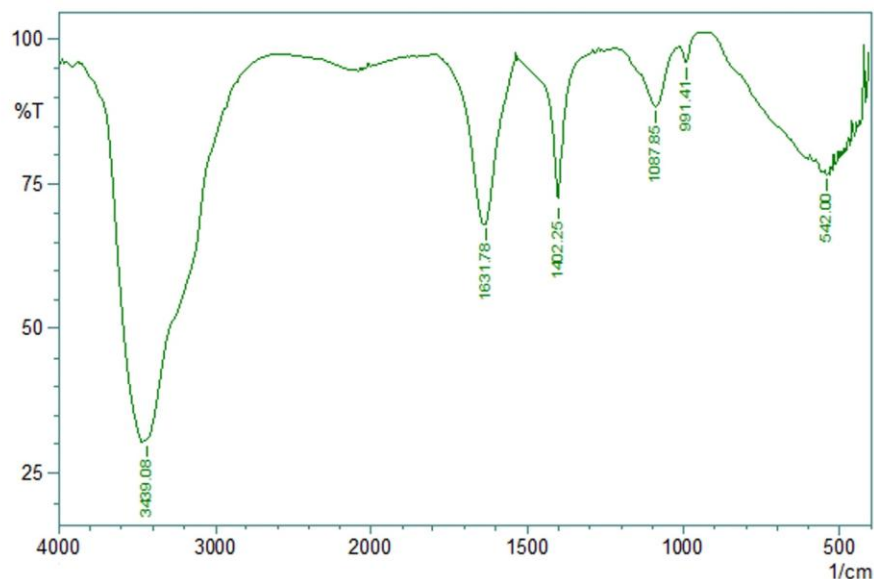
Fig. 4: FTIR spectra of AgNPs.
