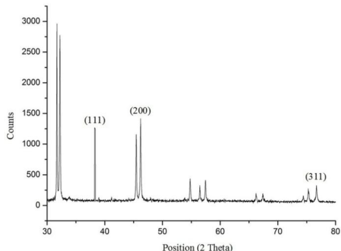
Fig. 7: Smoothen format of XRD pattern showing the presence of different peaks on 2 theta plane indicating the crystalline structure of the synthesized AgNPs.
