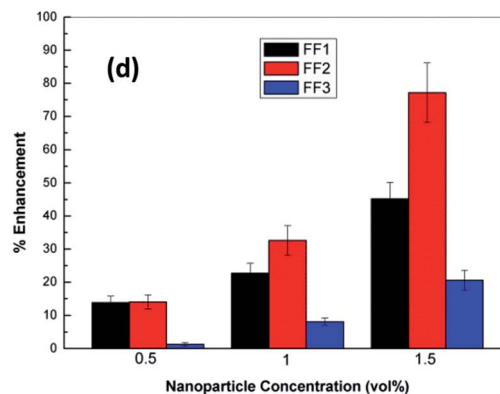
Fig. 7 Variation of co-efficient of thermal conduction as a function of \gamma - \text{Fe}_2\text{O}_3 nanoparticles concentration in (a) liquid paraffin (b) motor (c) sunflower oil base fluid. (d) Variation of % enhancement of thermal conductivity as a function of \gamma - \text{Fe}_2\text{O}_3 nanoparticles concentration.
