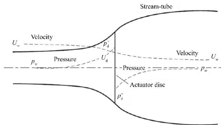
Figure 2. An energy extracting actuator disc and stream tube.
