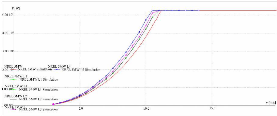
Figure 3. Graphical summary of simulation for variation in radius.
