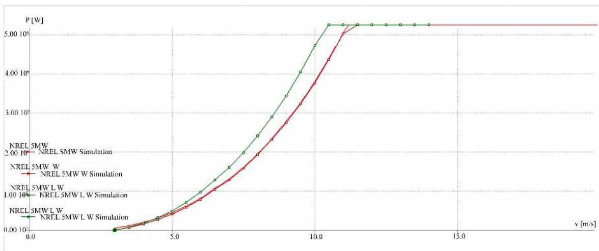
Figure 4. Summarizes change in power output for variation in chord of the blade proportion to the radius and also for varying the chord alone.
