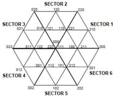
Fig 3. Space vector modulation three level NPC inverter
