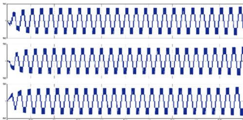
Fig 6. Three Level NPC Inverter output
