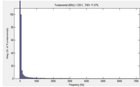
Fig 9. THD VOC PI controller (17.47%)
