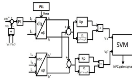
Fig 5. VOC PR controller
