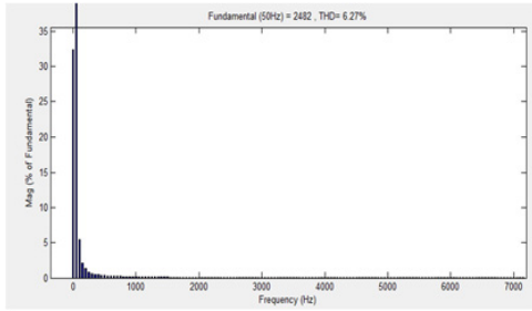
Fig 8. THD VOC PR controller (6.27%)
