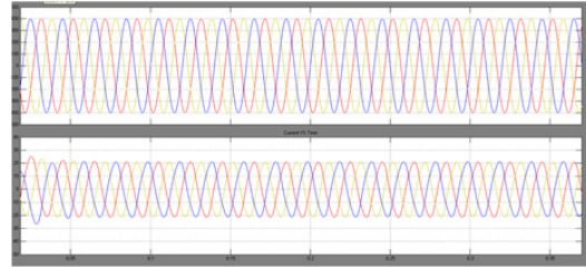
Fig 7. Grid voltage and Grid current
