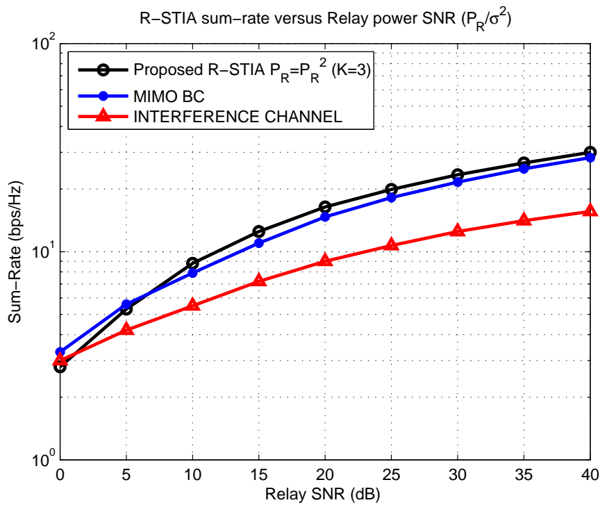
Figure 8. Sum-rate for the proposed relay space-time interference alignment (R-STIA) technique.
