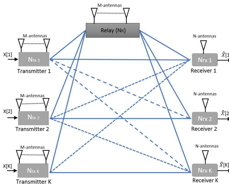
Figure 1. The K -user multiple-input-multiple-output (MIMO) interference channel model with a shared relay.
