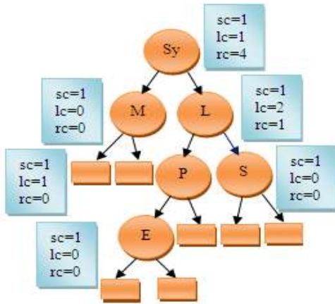
Fig. 10: Initial lazy counting-based splay tree with aspects
