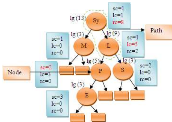
Fig. 11: Injection of persistence aspect
