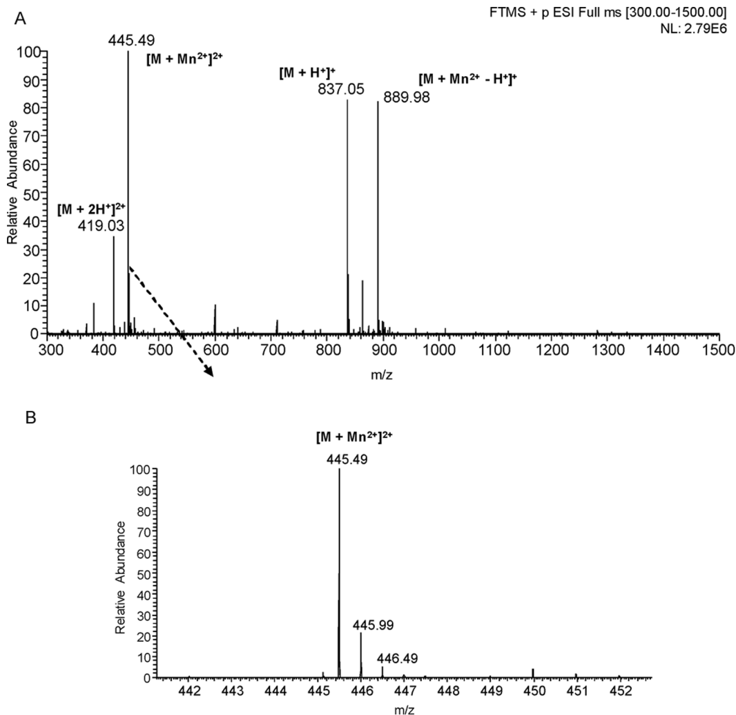
Figure 3. Detection of the intermediate 'I' of the DAC assay. (A) LC - ESI -MS spectrum showing the peaks corresponding to proton and manganese ion adducts of the intermediate 'I' of molecular mass 836 Da. (B) Expansion of the region, m/z 442–452 of the spectrum shown in (A); m/z values and intensity distribution of isotope peaks indicating doubly charged manganese ion adduct of 'I'. doi:10.1371/journal.pone.0086096.g003
