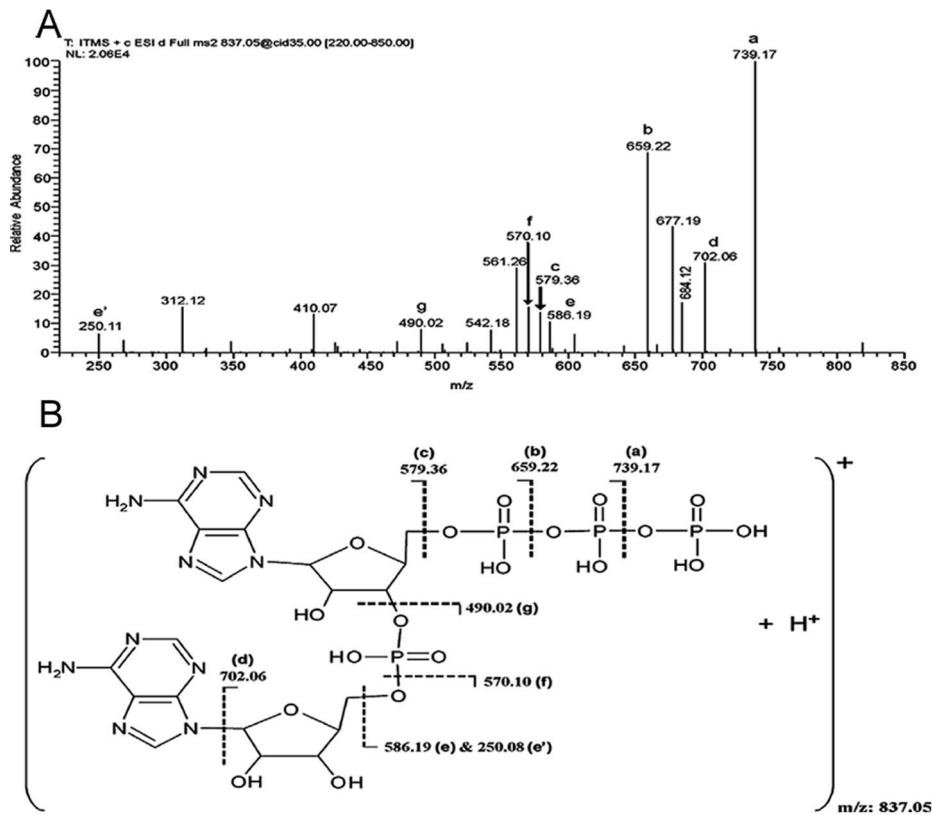
Figure 4. Reaction intermediate 'I' was determined to be pppApA. (A) LC-ESI-MS/MS spectrum of [M+H]^+ precursor ion m/z 837.05 (reaction intermediate 'I'). (B) Figure depicting the interpretation of the fragmentation as observed in (A). doi:10.1371/journal.pone.0086096.g004
