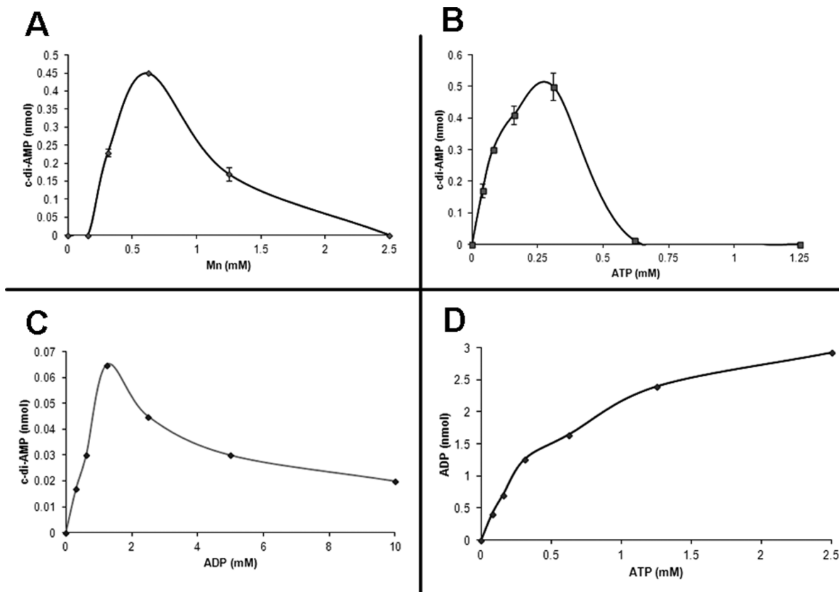
Figure 2. DAC activity is regulated by ATP. (A) Optimum Mn^{2+} concentration. The optimum concentration of Mn^{2+} was determined by doing the assay (20 \mu l) in presence of 25 mM Tris-HCl (8.5), 25 mM NaCl, 300 \mu M ATP, 1 \mu M of MtbDisA, varying concentrations of MnCl_2 and the reaction was incubated at 37°C for 15 min. The plot shows the amount (nmoles) of c-di-AMP formed during the reaction as a function of Mn^{2+} concentration (B) ATP dependence. The extent of formation of c-di-AMP in 20 \mu l reaction mixtures was determined by doing the DAC assay in presence of 25 mM Tris-HCl (8.5), 0.6 mM Mn^{2+} , 25 mM NaCl, 1 \mu M of MtbDisA and different concentrations of ATP. The reaction mixtures were incubated at 37°C for 15 min. The plot shows the formation of c-di-AMP as a function of ATP concentration. The data plotted in (A) and (B) represent the mean of three independent experiments \pm standard deviation. (C) ADP inhibition. The DAC assay was carried out in 10 \mu l reaction mixtures containing 25 mM Tris-HCl (pH 8.5), 0.6 mM MnCl_2 , increasing concentrations of ADP as indicated, 2 \mu M of MtbDisA and incubated for 15 min at 37°C. The reaction mixtures were processed and analyzed as before. The plot shows the formation of c-di-AMP as a function of ADP concentration. (D) D72AG73A has ATPase activity. The DAC assay was carried out in 10 \mu l reaction mixtures containing 25 mM Tris-HCl (pH 8.5), 0.6 mM MnCl_2 , indicated concentrations of ATP, 2 \mu M of D72AG73A and incubated for 30 min at 37°C. The reaction mixtures were processed and analyzed as before. The plot shows the formation of ADP as a function of ATP concentration. doi:10.1371/journal.pone.0086096.g002
