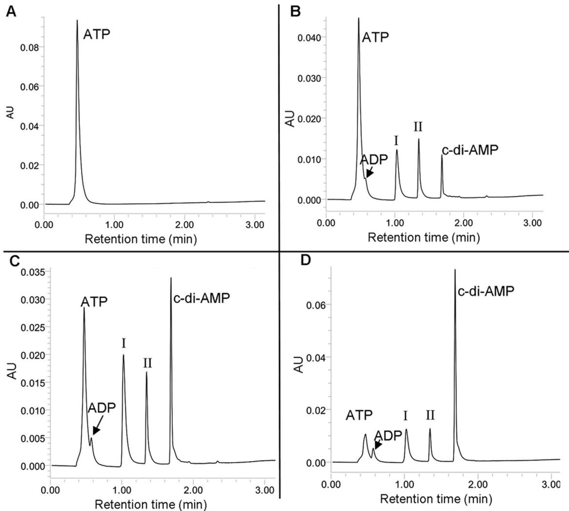
Figure 1. MtbDisA synthesizes c-di-AMP through two intermediates. DAC assay was done in 10 \mu l reaction mixtures containing 25 mM Tris-HCl (pH 8.5), 0.6 mM MnCl_2 , 300 \mu M ATP and 2 \mu M of MtbDisA and incubated at 37°C. The reaction mixture was subjected to reverse phase LC and the products were detected with UV ( \lambda 260 nm). The absorption chromatograms with peaks labeled with the corresponding species have been shown. (A) Peak for only ATP is detected in the control reaction (without enzyme). ATP is converted into c-di-AMP in the presence of MtbDisA as can be seen in (B). Two more peaks are detected in 'B' which are the intermediates of the reaction and are labeled 'I' and 'II'. In (B) the DAC reaction was terminated after 5 min whereas in (C) and (D) the reaction was continued for 10 and 60 min respectively. Peak for ADP has been labeled. doi:10.1371/journal.pone.0086096.g001
