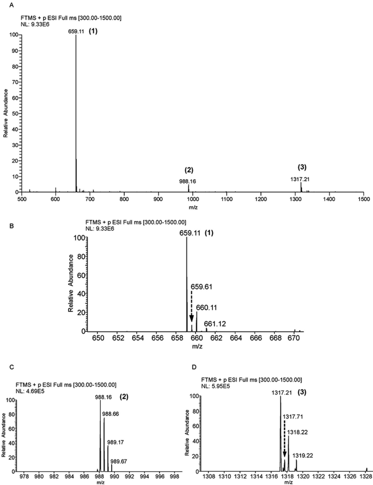
Figure 5. Two-step synthesis of c-di-AMP. The figure shows the formation of c-di-AMP from the two intermediates pppApA and ppApA. pppApA is first formed by conjugation between two molecules of ATP (step 1A). Two ADP molecules or one molecule of ADP and one ATP molecule can conjugate to give rise to ppApA (step 2A). pppApA and ppApA are then converted into c-di-AMP (steps 1B & 2B) through their respective Mn^{2+} -adduct (transition state complex) as shown. doi:10.1371/journal.pone.0086096.g005
