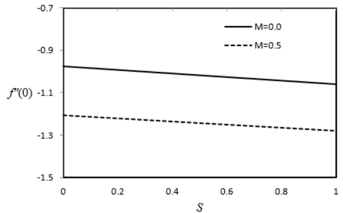
Fig. 12 Surface skinfriction versus S for different M
