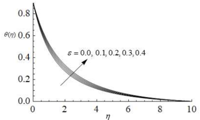
Fig. 11 Temperature profiles for different values of \varepsilon
