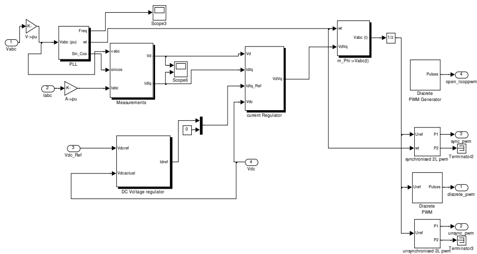
Fig. 5. Network bridge control block
