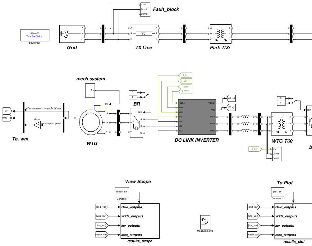
Fig. 1. Top Level Wind Farm Model
