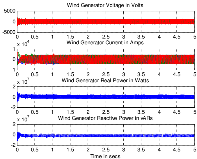
Fig. 12. Generator-side electrical outputs, normal operation
