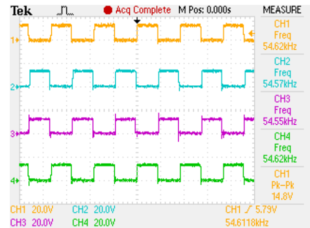
Figure 7. Gate Pulses from IR2110 driver.
