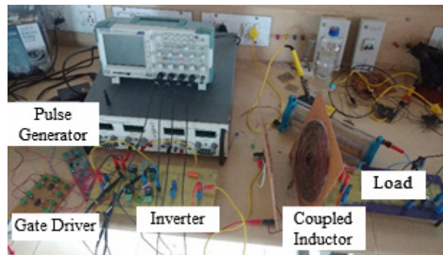
Figure 6. Photograph of the experimental setup.
