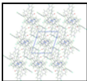
Fig. 3. A view in projection down the c axis of the unit-cell contents of (I). The C—H \cdots \pi , \pi - \pi , and C—Cl \cdots \pi interactions are shown as purple, orange and green dashed lines, respectively.
