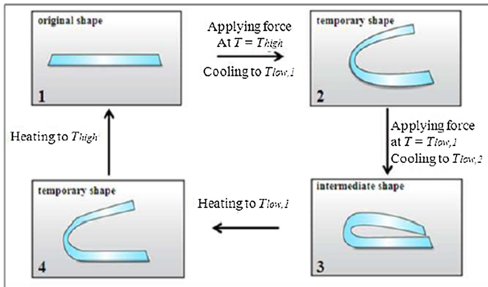
Fig. 13. Triple shape memory effect. (Reproduced from [112]).
