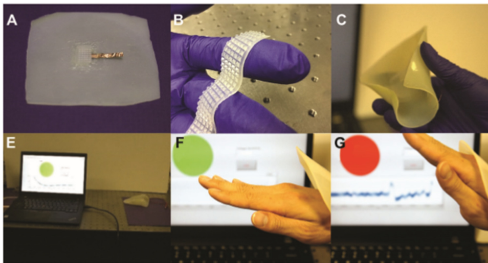
Fig. 23. STENG shape-changing wrist splint. (Reprinted with permission from [173], Copyright with License Number: 4630111089845).
