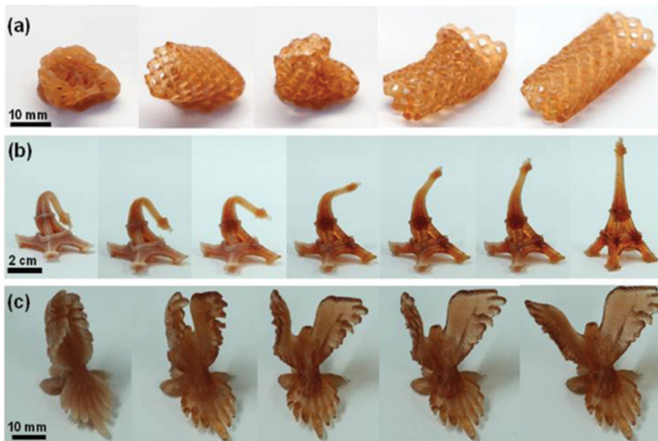
Fig. 9. Shape changing structures printed using SLA. (Reprinted with permission from [95], Copyright with License Number: 4615880573475).
