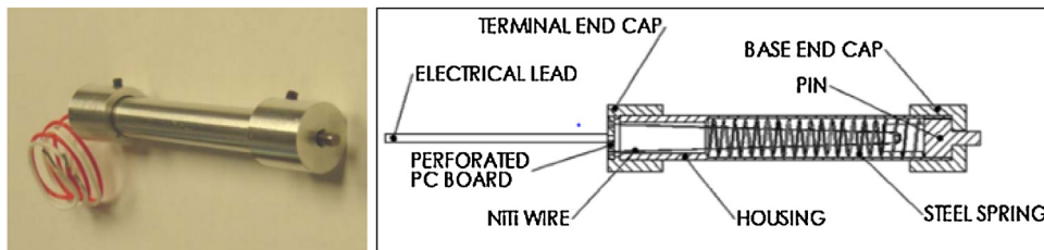
Fig. 4. SMA based pin puller for aerospace application.
