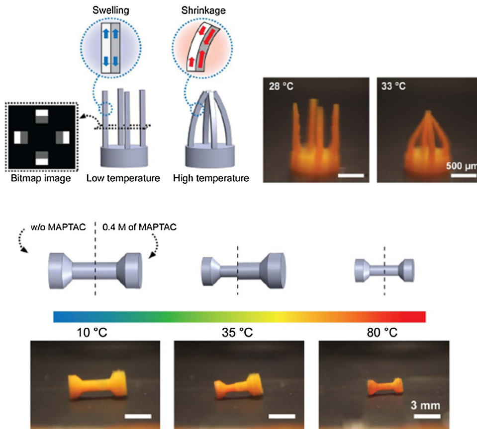
Fig. 7. PNIPAAm hydrogel-based structures.
