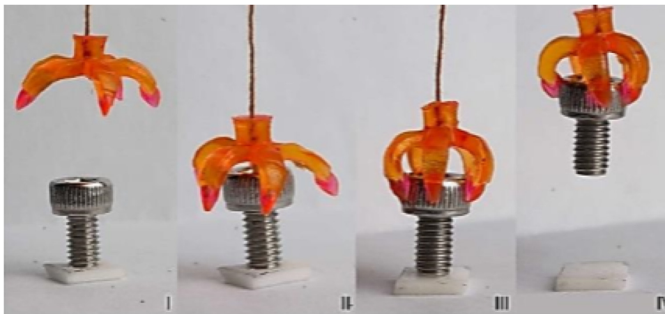
Fig. 24. Heat actuated soft robotic grippers. (Reproduced from [99]).
