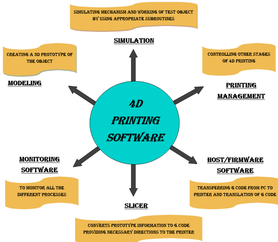
Fig. 3. 4D Printing software and their applications.
