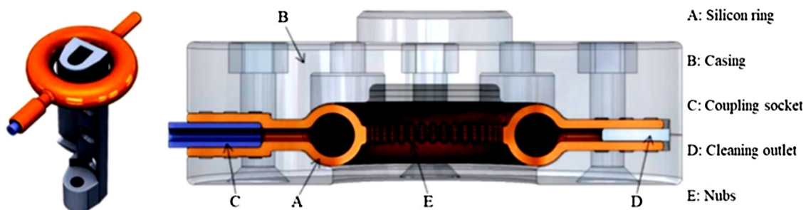
Fig. 25. Soft Robotic ring gripper. (Reprinted with permission from [178], Copyright with License Number: 4630111309171).
