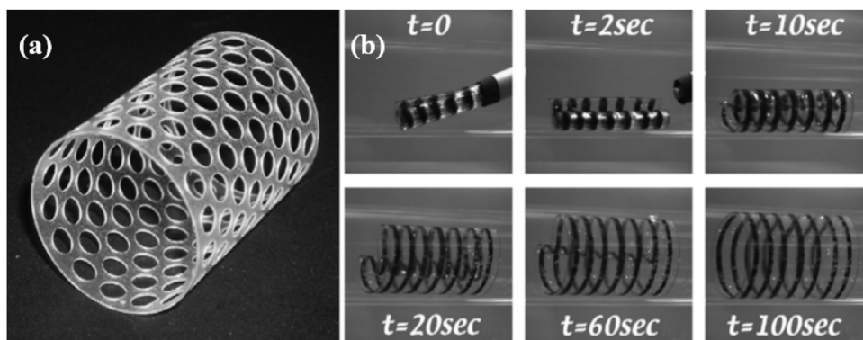
Fig. 18. (a) Perforated SMP stent (b) SMP stent-catheter system. (Reprinted with permission from [138], Copyright with License Number: 4615891002938).
