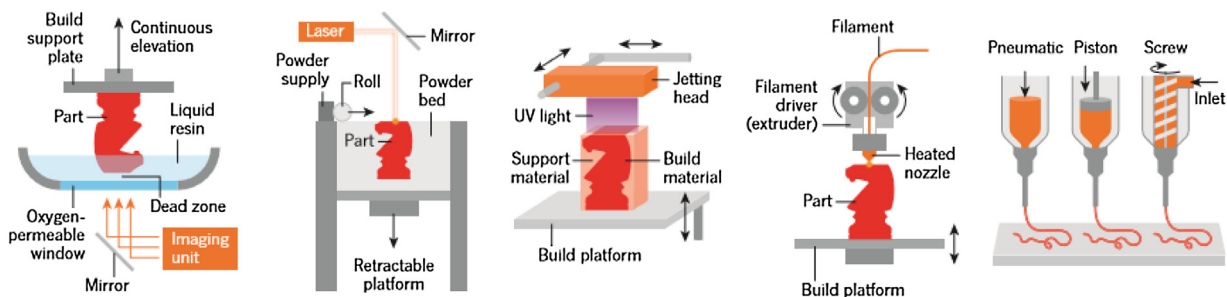
Fig. 8. Traditional light and ink-based 3D printing methods. (Reprinted with permission from [81], Copyright with License Number: 4615880329578).
