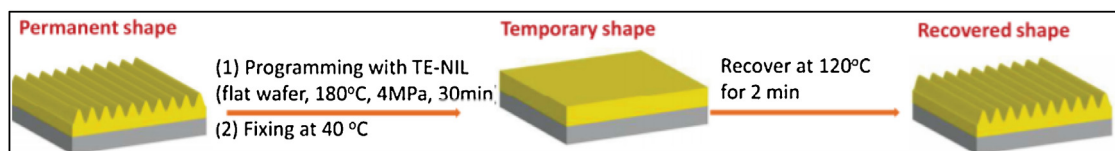
Fig. 6. Shape memory cycle of acrylate-based SMP.
