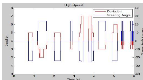
Figure 13. Test results on High speed
