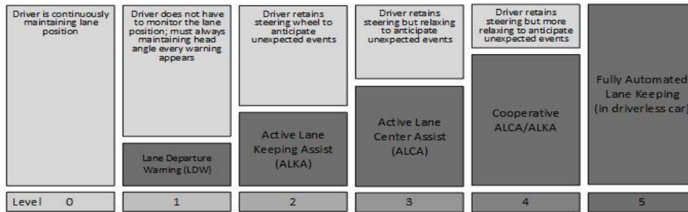
Figure 1. Level of automation LKA
