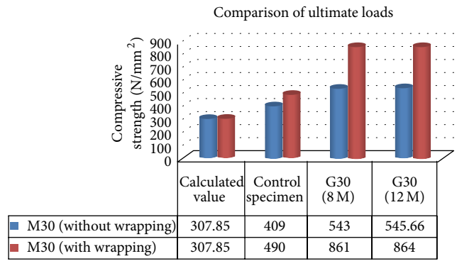
FIGURE 3: Comparisons of ultimate loads.
