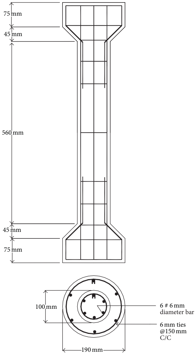
FIGURE 1: Reinforcement details.
