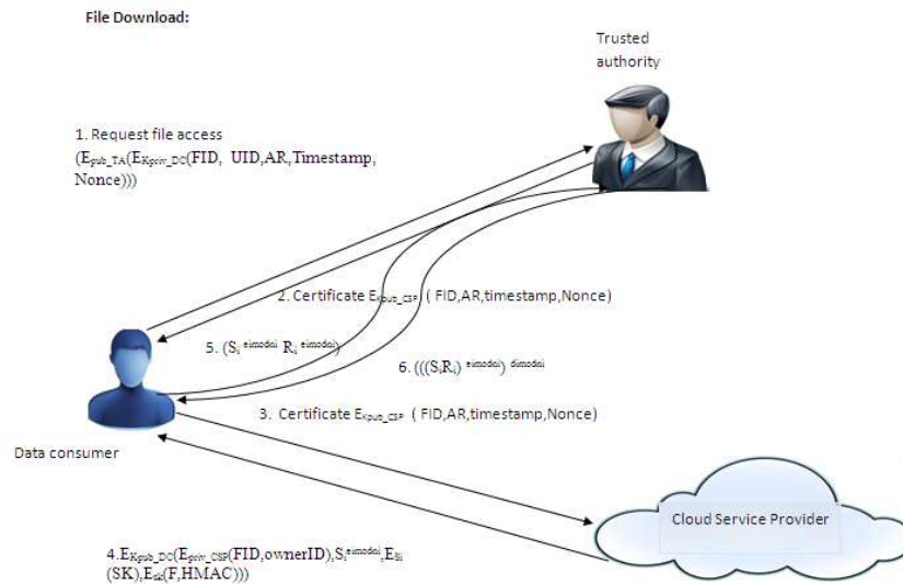
Figure 3 File Download.
