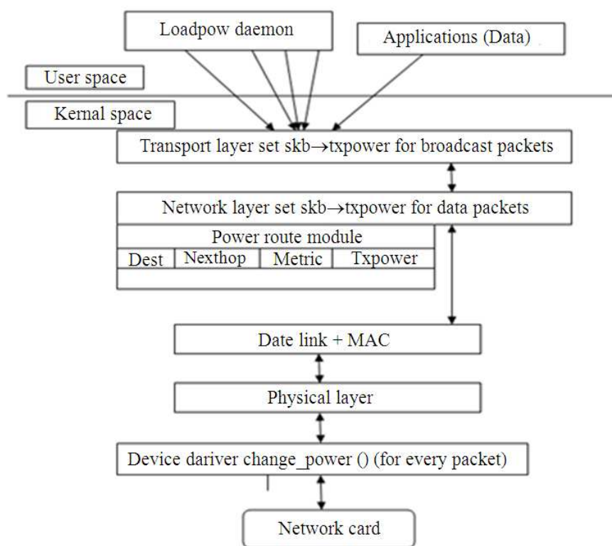
Fig. 4. Load power architecture
