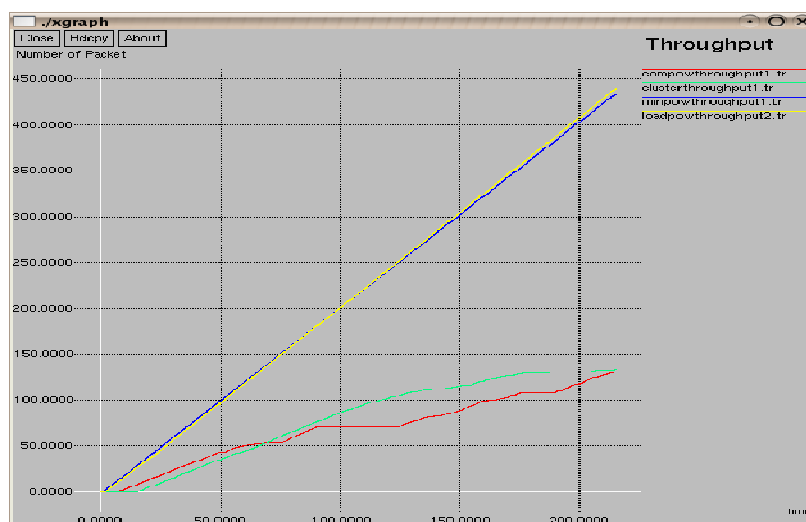
Fig. 5. Throughputs for four protocols
